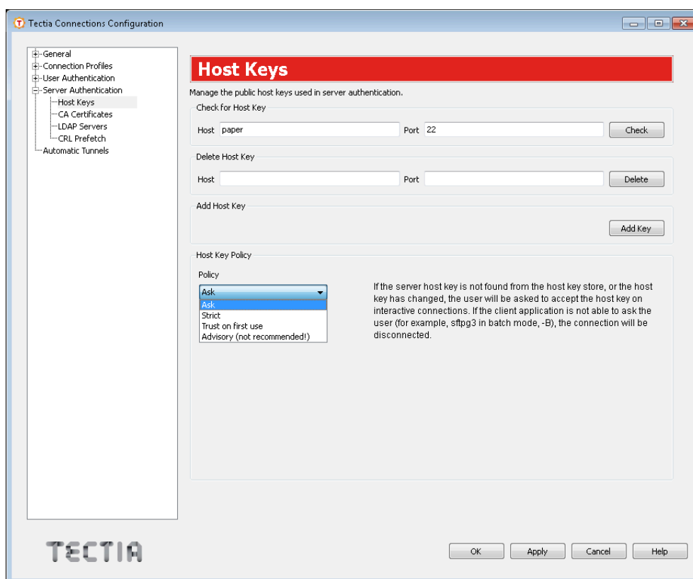
Figure A.37. Defining server host keys settings
