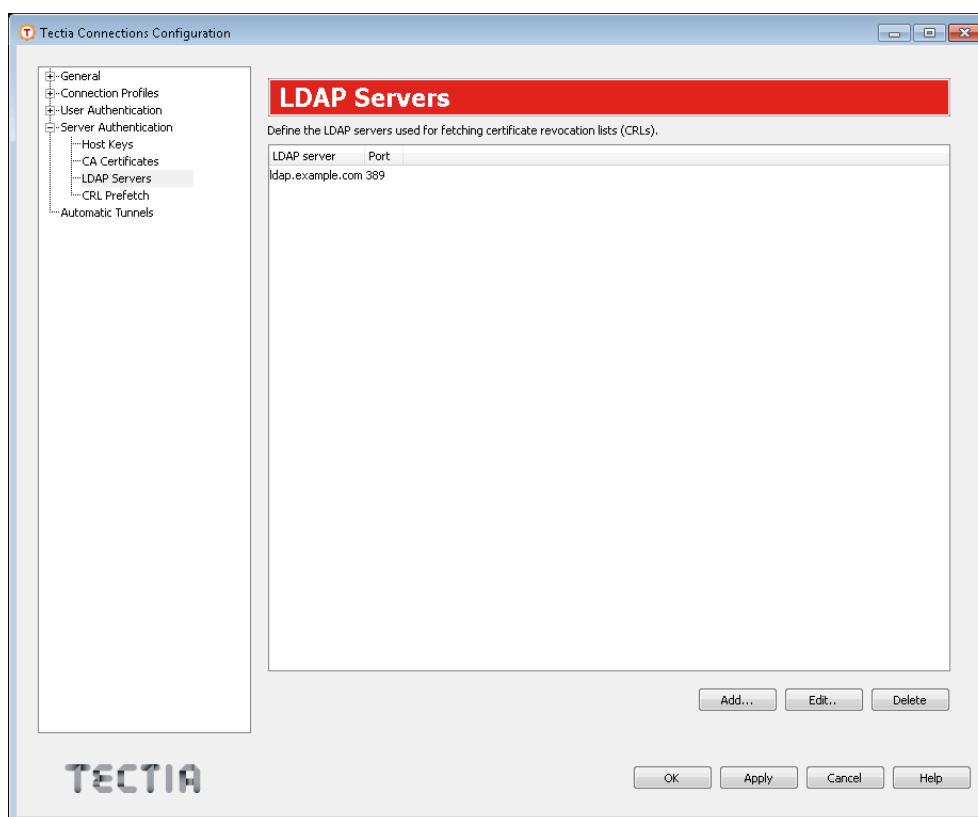
Figure A.40. Defining LDAP servers
